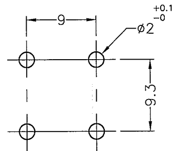
MOUNTING HOLE
