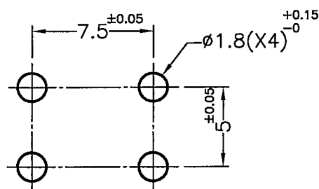
MOUNTING HOLE
