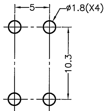
MOUNTING HOLE
