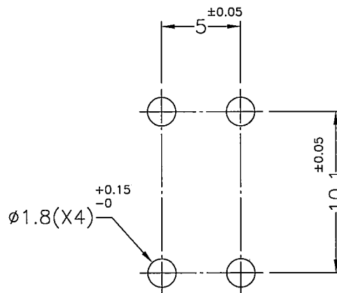
MOUNTING HOLE
