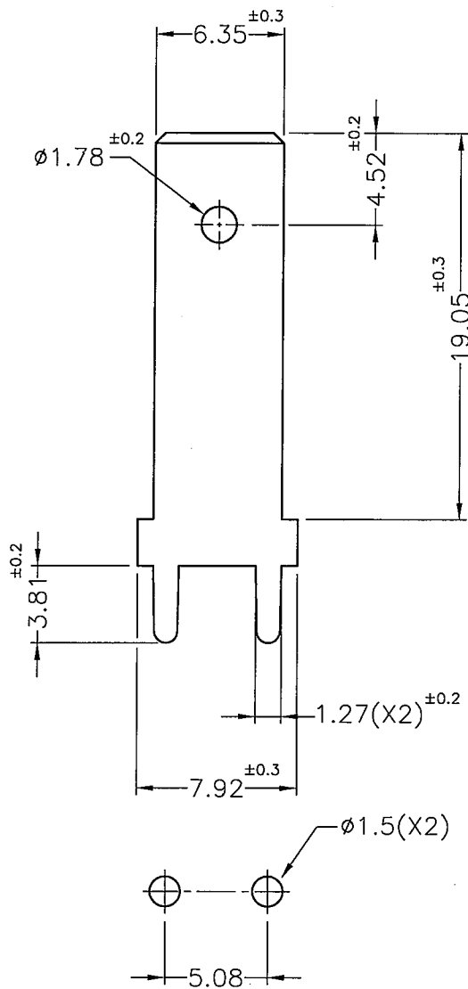
MOUNTING HOLE
