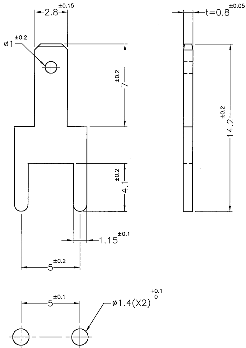
MOUNTING HOLE
