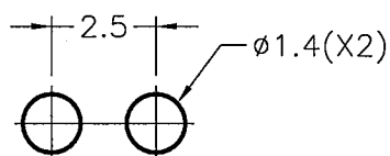
MOUNTING HOLE
