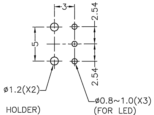
MOUNTING HOLE
