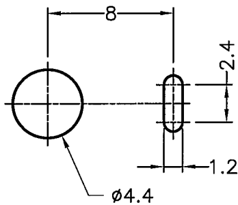
MOUNTING HOLE
