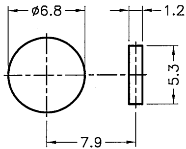
MOUNTING HOLE
