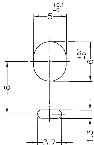
MOUNTING HOLE
