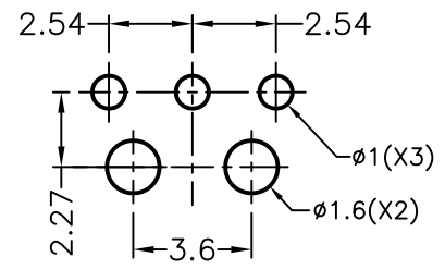
MOUNTING HOLES
