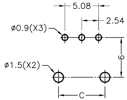
MOUNTING HOLES
