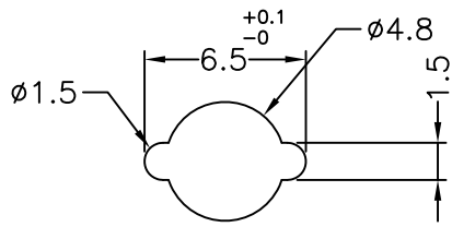
MOUNTING HOLE
