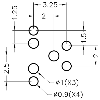
MOUNTING HOLES
