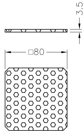
FANCV-5C
