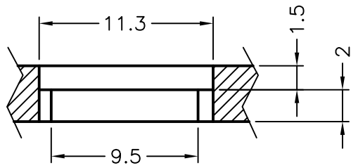
MOUNTING HOLE
