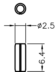
PIN
