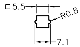
MOUNTING HOLE
